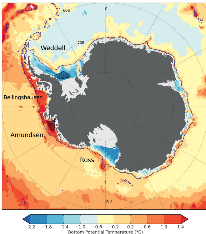
FIG. 1. Map of the Southern Ocean bottom potential temperature. Ocean data are from the WOCE global hydrographic climatology (Gouretski and Koltermann 2004). The reference study regions are shown by the black hatched boxes in the Weddell and Amundsen seas. The 1000-m bathymetry contour (dark blue line) and the Antarctic landmask are taken from the RTOPO dataset (Timmermann et al. 2010).
